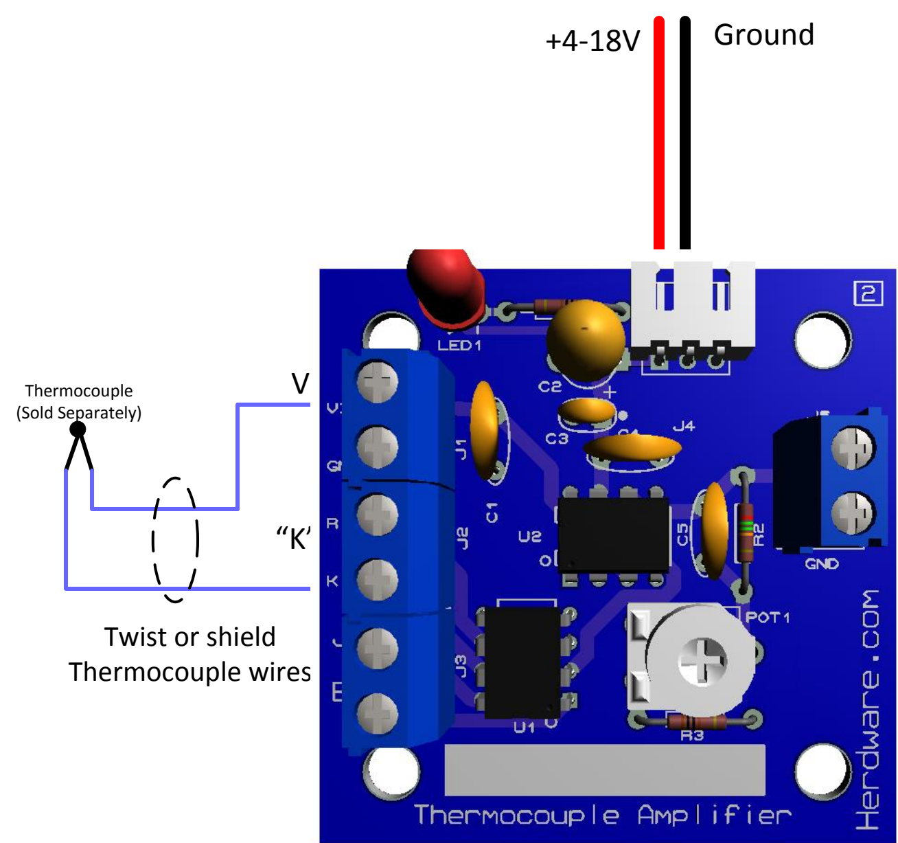
Wire Thermocouple between VIN and Terminal denoting type: Example Type K Shown
